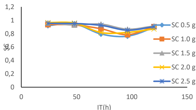
Figure 9: Dependence from \theta by MBZ on the IT of MS in 0.5 M \text{H}_2\text{SO}_4 .
