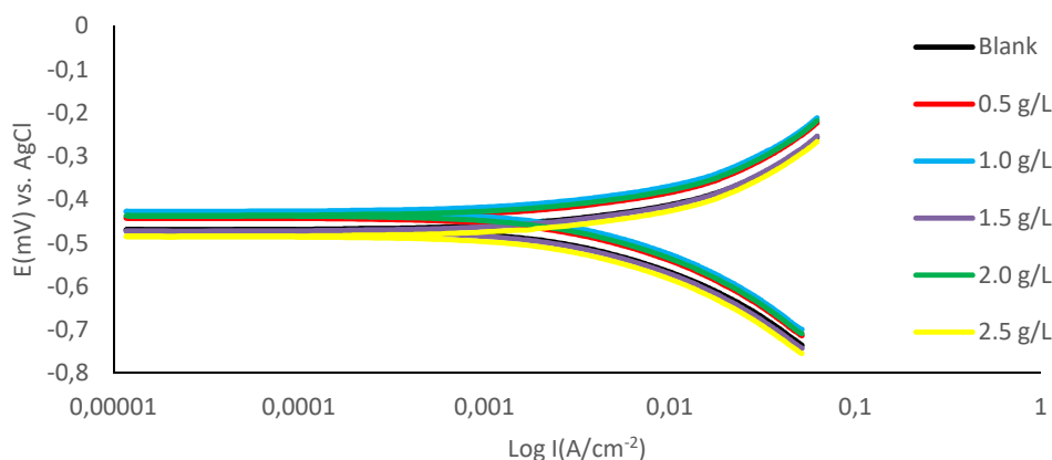
Figure 11: PDP curves for MS in 0.5 M \text{H}_2\text{SO}_4 without and with MBZ, in various C, at 303 K.
