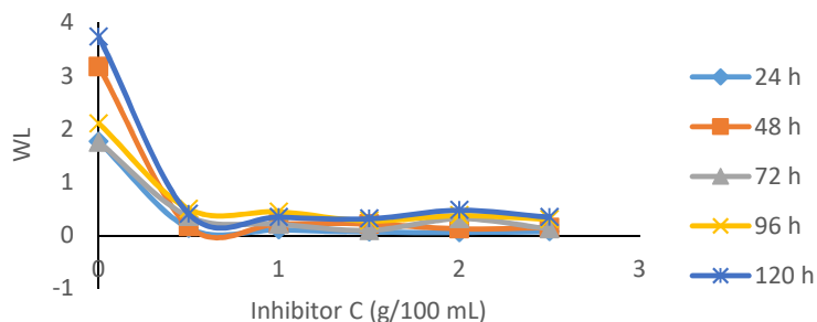
Figure 6: Dependence from WL of MS on C of MBZ.
