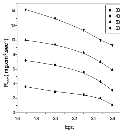
Figure 3. Corrosion rate of low carbon steel in 1 M HCl solution in the presence of different concentrations of compound 1 , at different temperatures.
