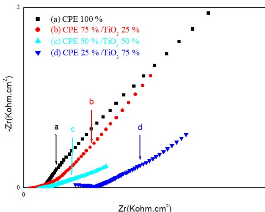
Figure 2: EIS diagrams recorded in 0.1 M NaCl alkaline medium at- (a) CPE 100%, (b) CPE 75%/TiO 2 25%, (c) CPE 50%/TiO 2 50% and (d) CPE 25%/TiO 2 75%.
