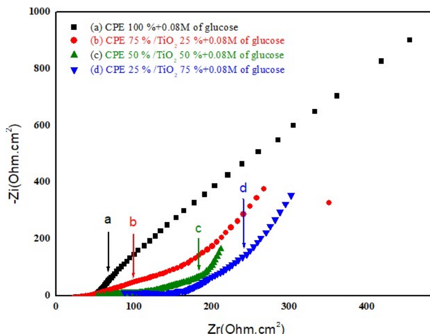
Figure 5: EIS recorded in 0.1 M NaCl alkaline medium containing 0.08 M glucose at (a) CPE 100%, (b) CPE 75%TiO 2 25%, (c) CPE50%TiO 2 50% and (d) CPE25%TiO 2 75%.
