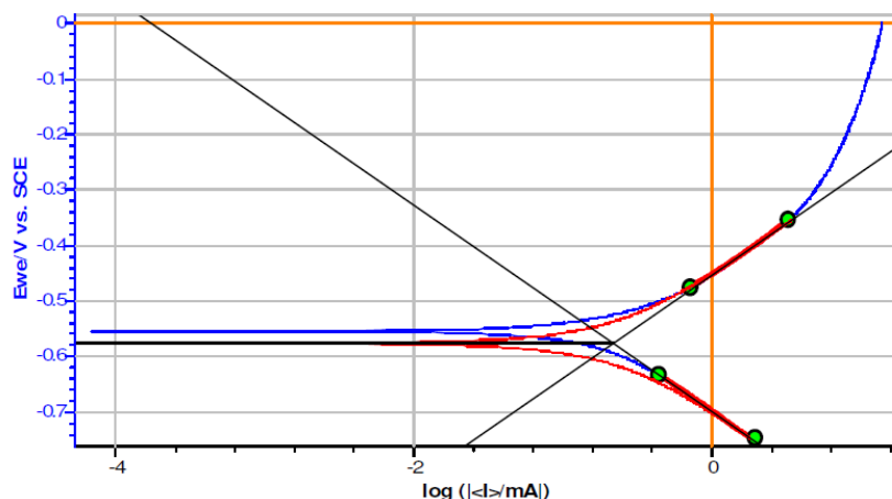
Figure 15. Potentiometric polarization curve for 0.5 M H 2 SO 4 medium, in the presence of 900 ppm concentration of Commelina benghalensis leaves extract.
