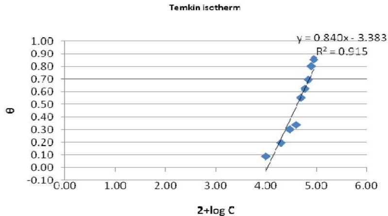
Figure 5. Temkin adsorption isotherm for mild steel corrosion inhibition in 0.5 M H 2 SO 4 , using Commelina benghalensis leaves extract.
